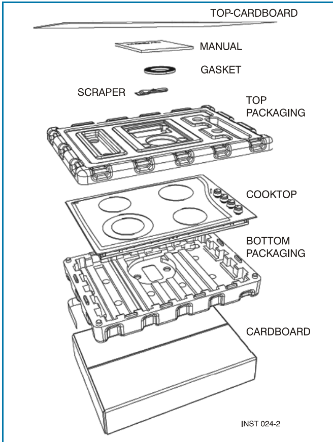
Figure 5. Parts
